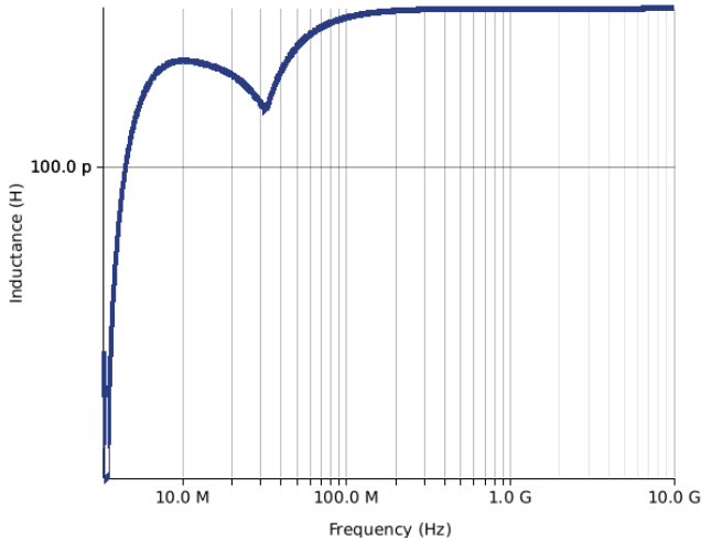
Inductance
