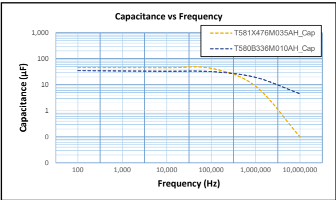
Capacitance vs. Frequency
