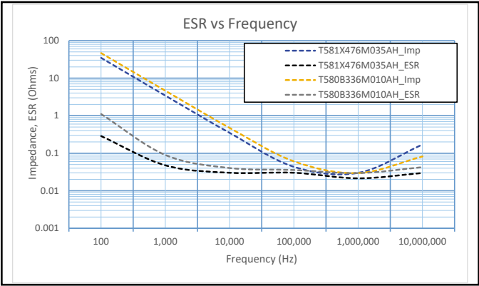
ESR vs. Frequency
