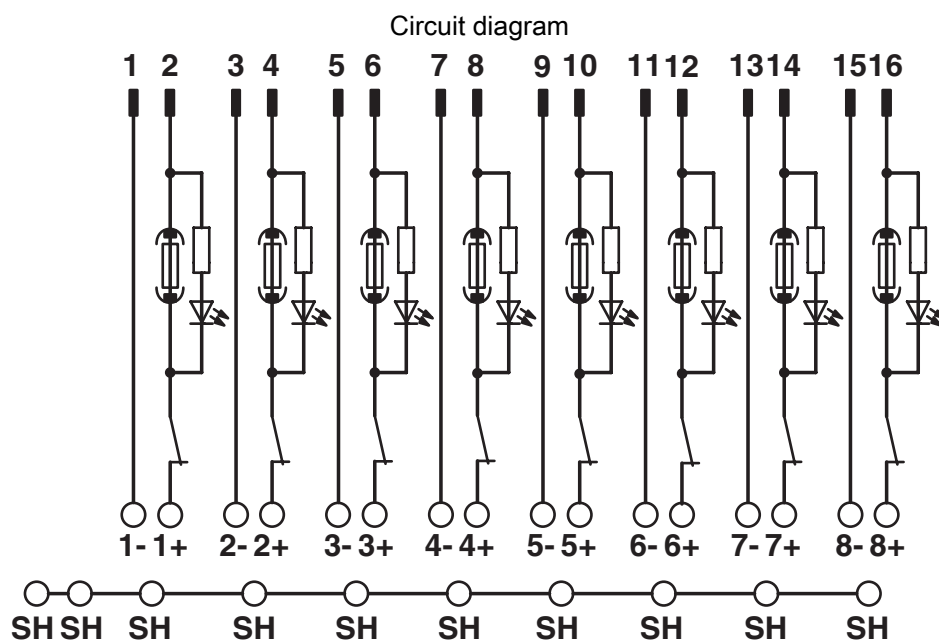
Connection scheme UM-DELTAV/A/SI/BFI/TP
