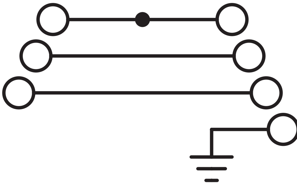
Circuit diagram
