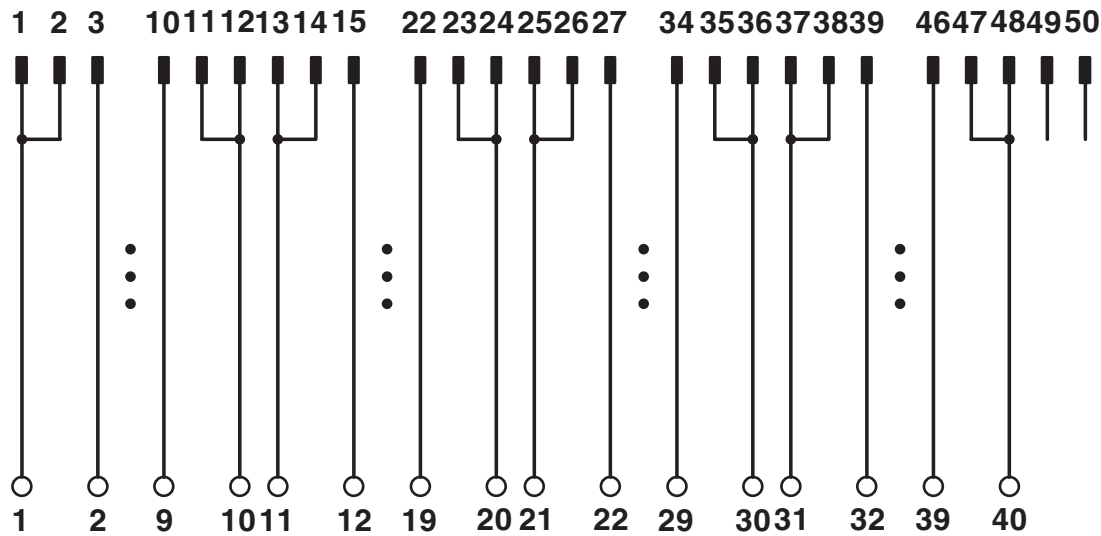
UM 45-FLK50/ZFKDS/S7-300 connection scheme
