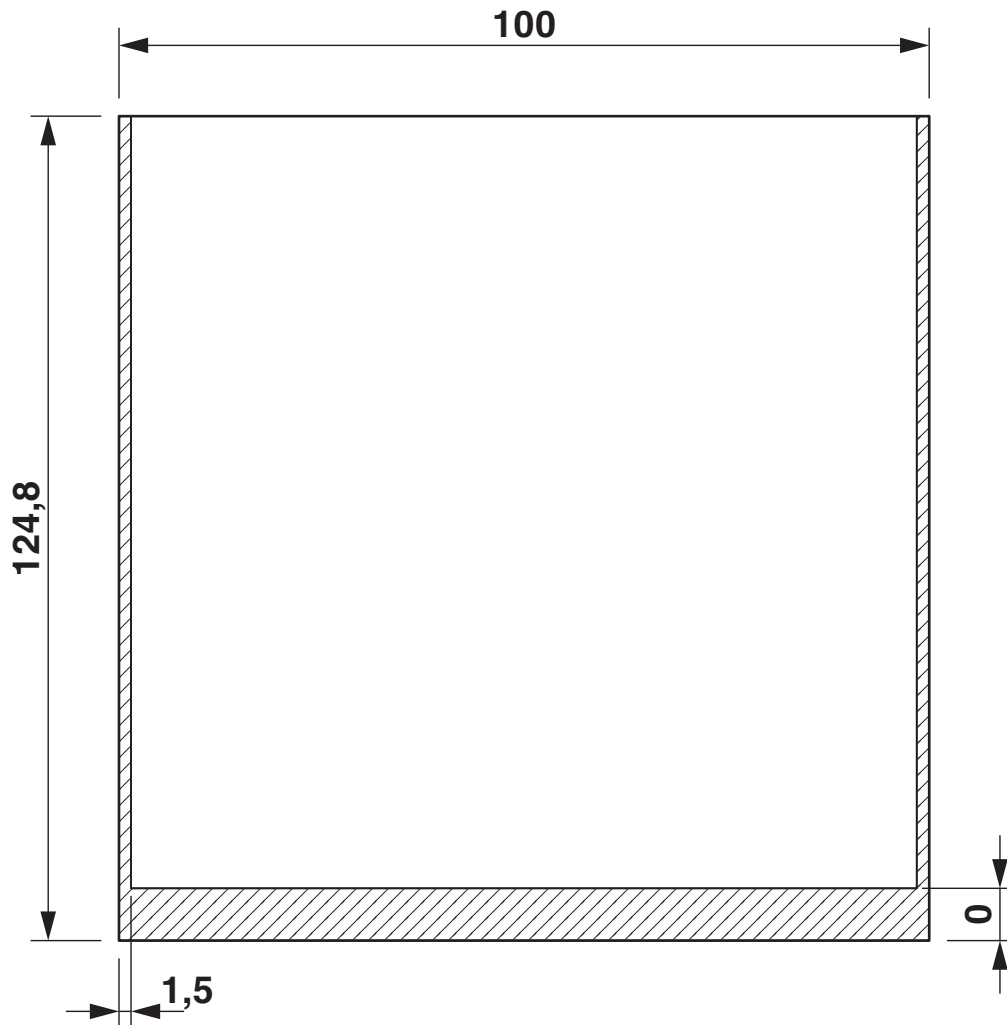
Dimensional drawing
