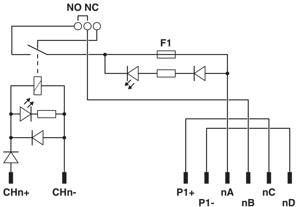
Circuit diagram
