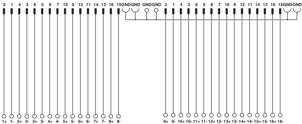
Circuit diagram
