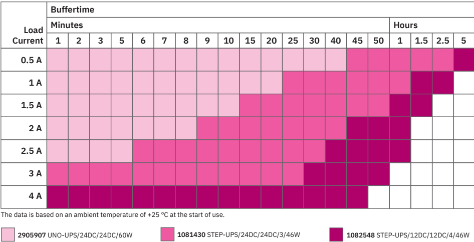
Buffer times for UNO DC UPS with integrated battery
