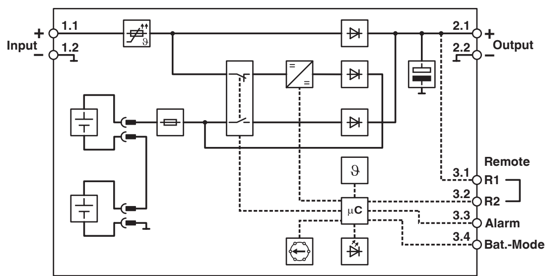
Block diagram
