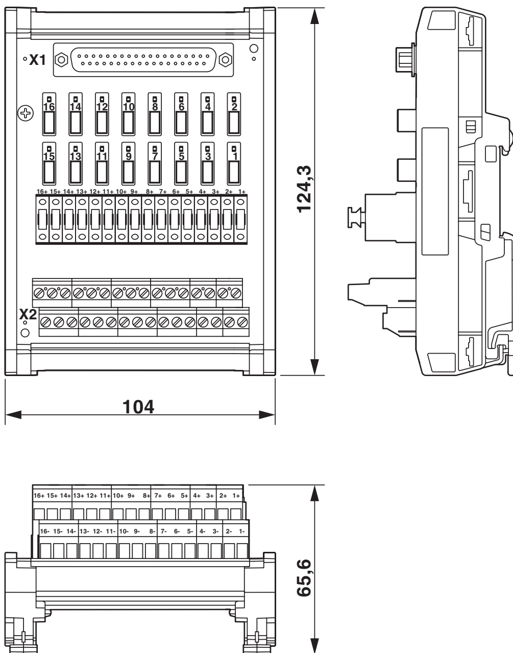
Dimensional drawing
