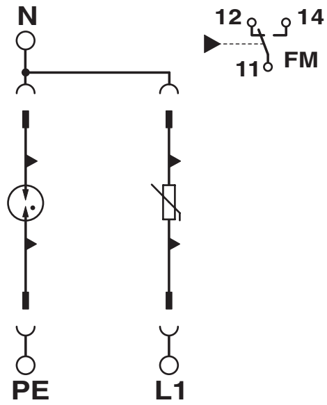
Circuit diagram
