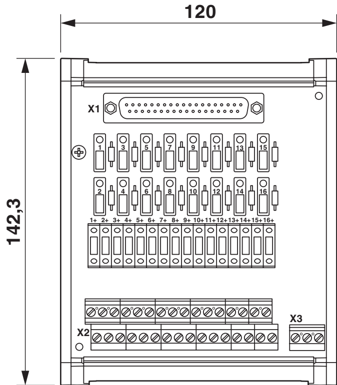
Dimensional drawing
