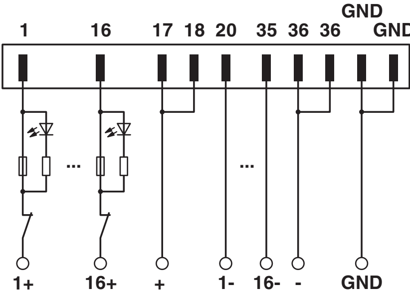
Circuit diagram
