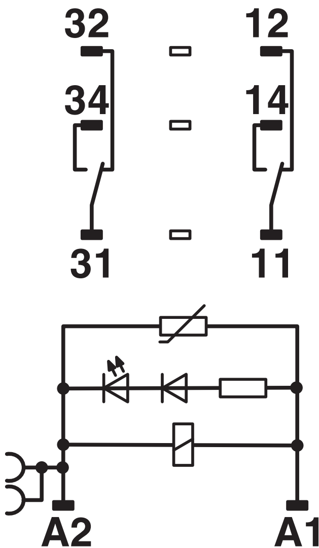
Circuit diagram
