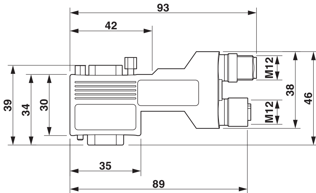
Application drawing
