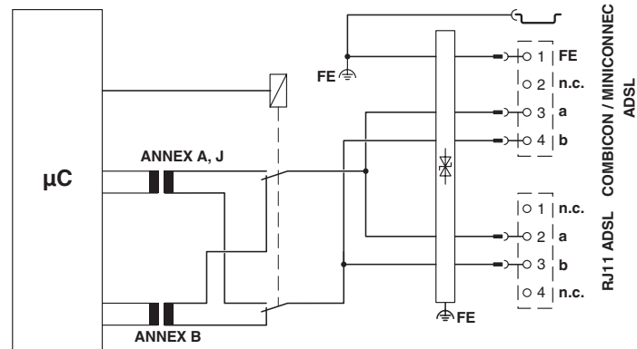
Circuit diagram
