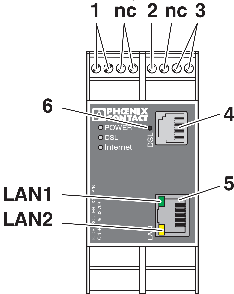
Schematic diagram
