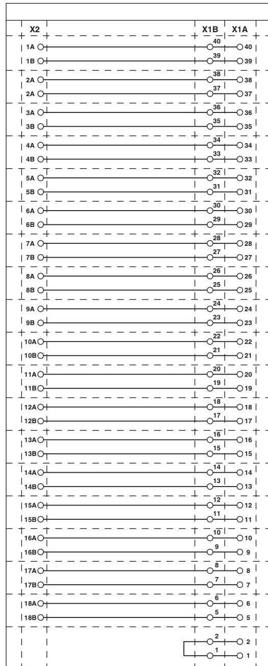
Circuit diagram
