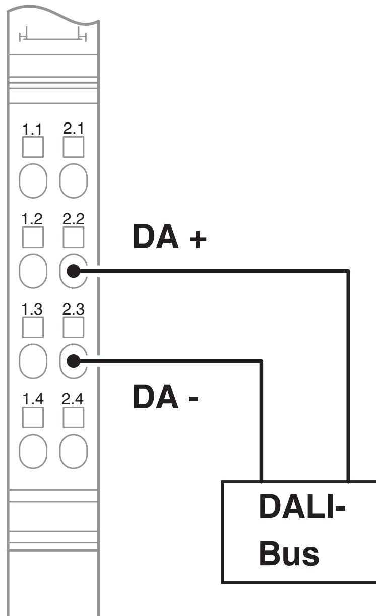
Connection diagram
