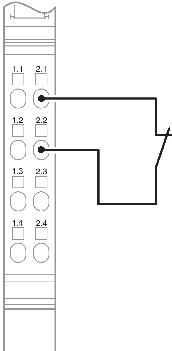
Connection diagram
