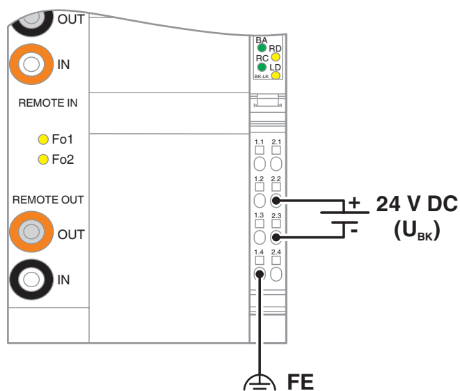
Connection diagram
