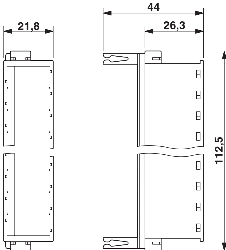
Dimensional drawing
