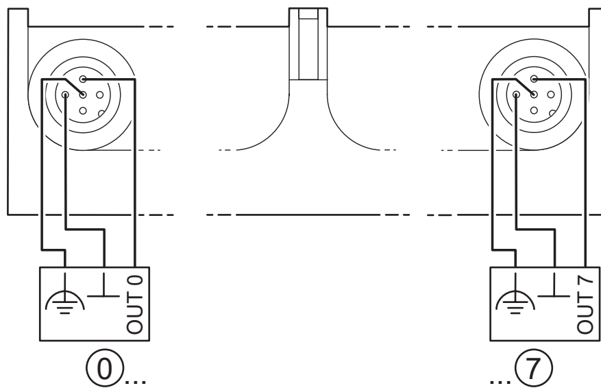
Connection diagram
