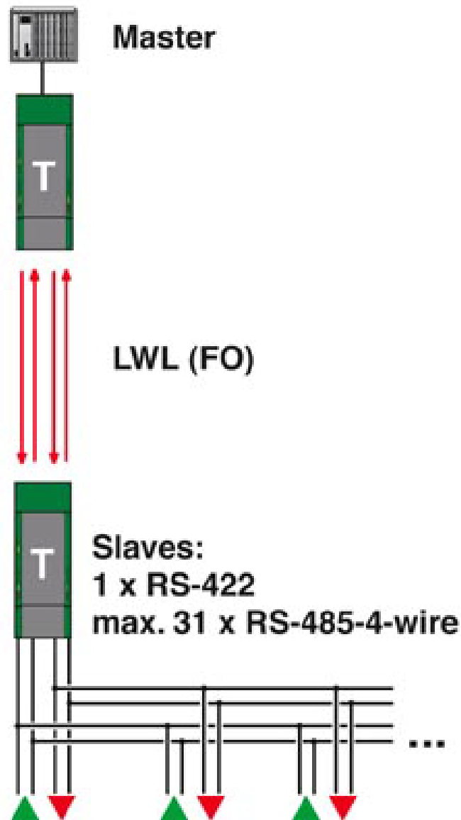
Application drawing
