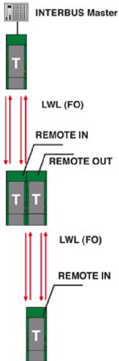
Application drawing
