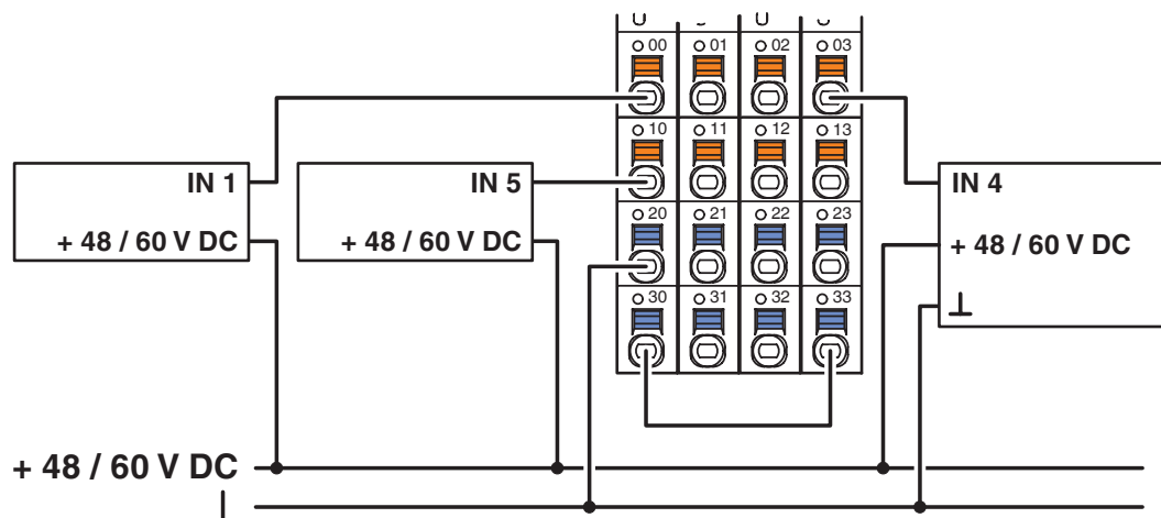
Connection diagram
