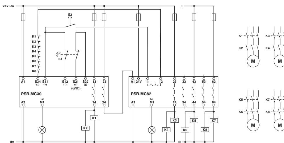
Circuit diagram
