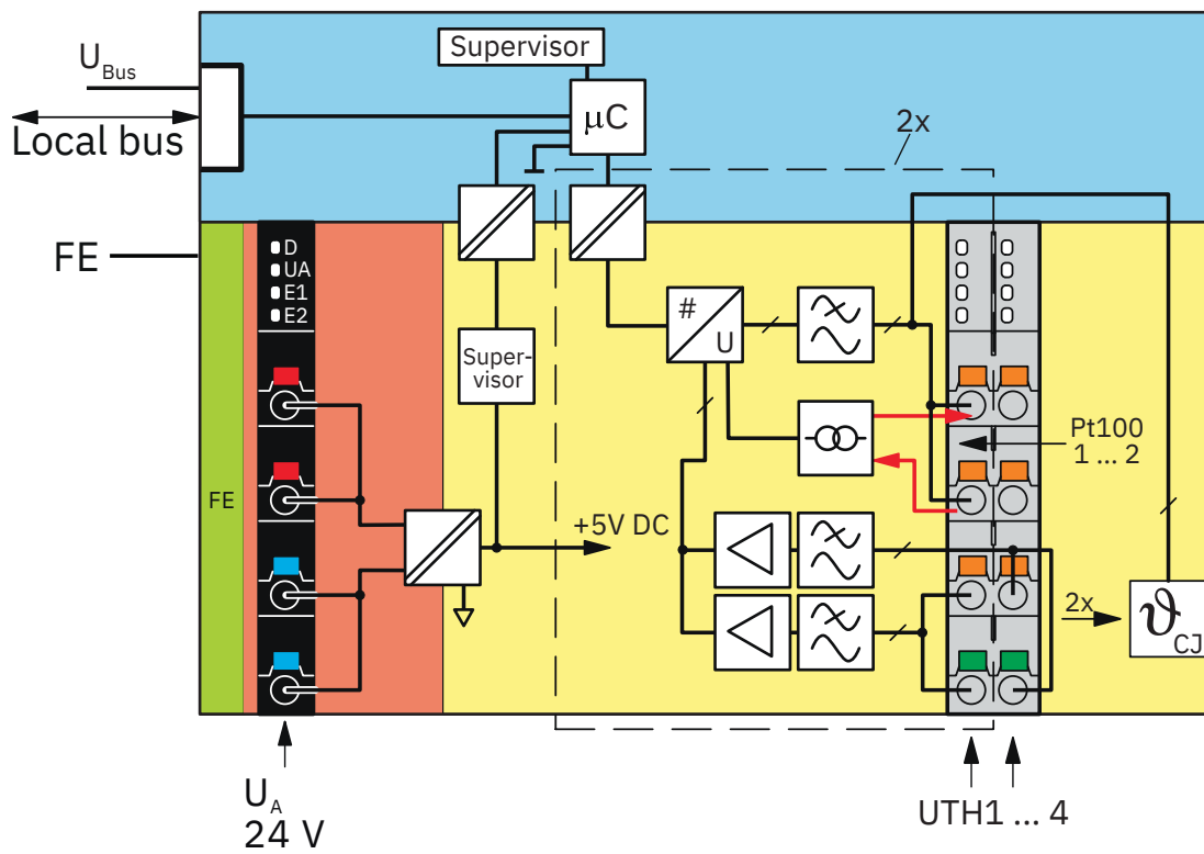
Block diagram
