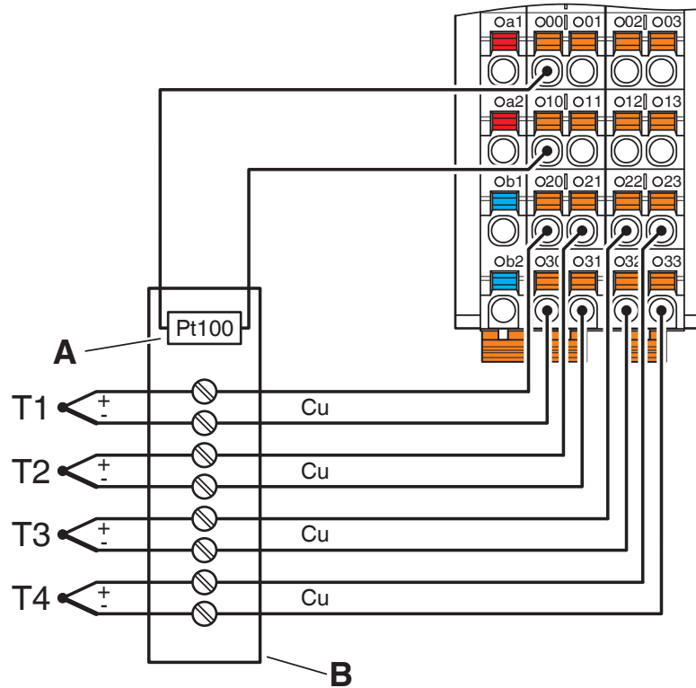
Connection diagram
