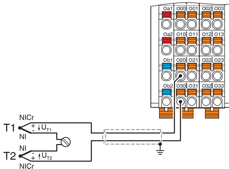
Connection diagram
