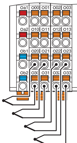
Connection diagram
