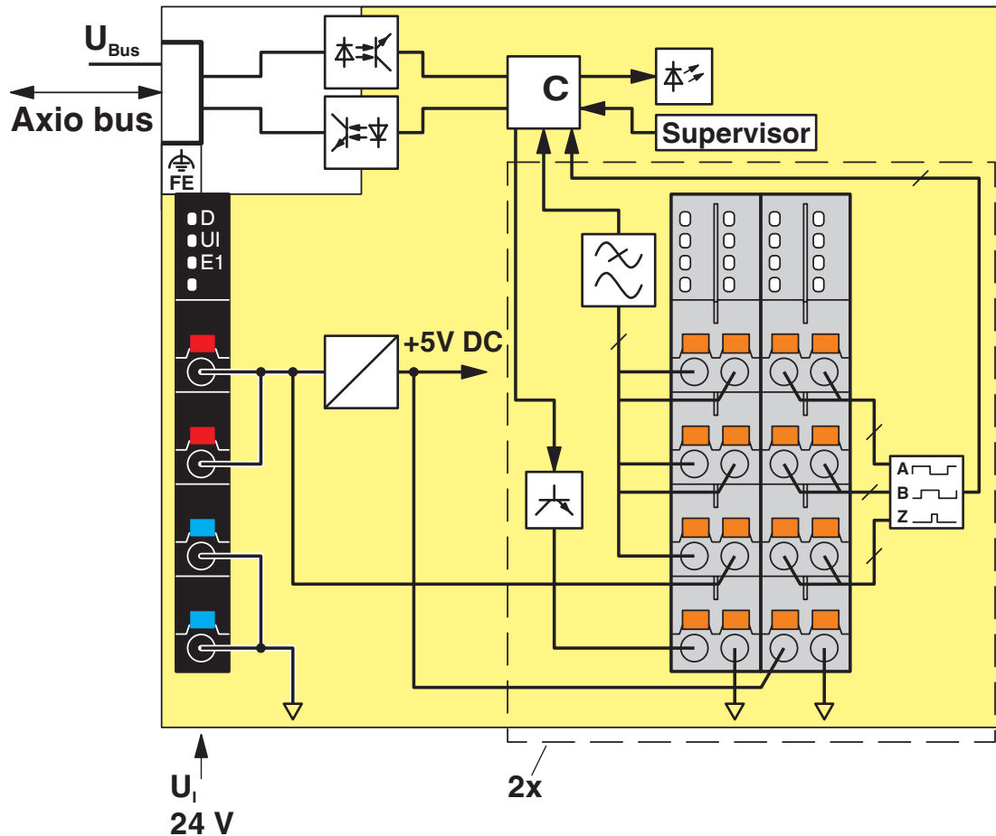
Block diagram
