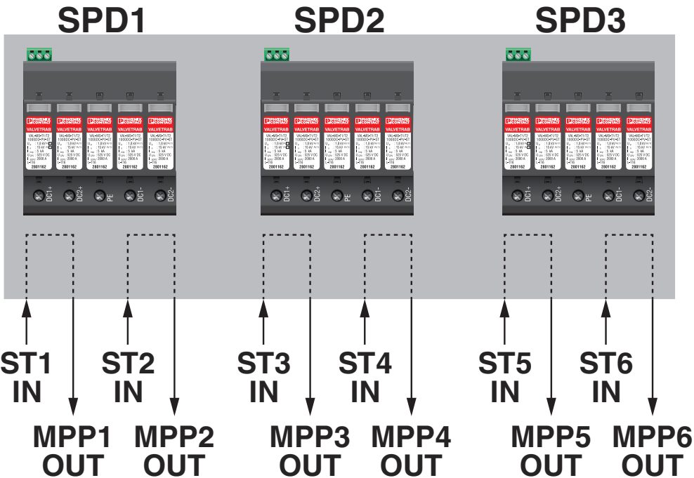
Connection diagram
