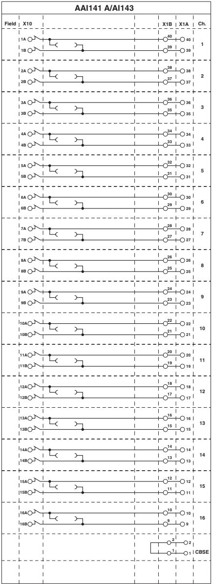
Circuit diagram
