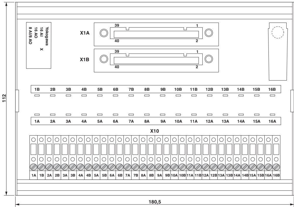
Dimensional drawing
