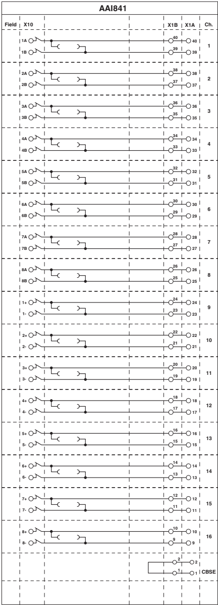
Circuit diagram
