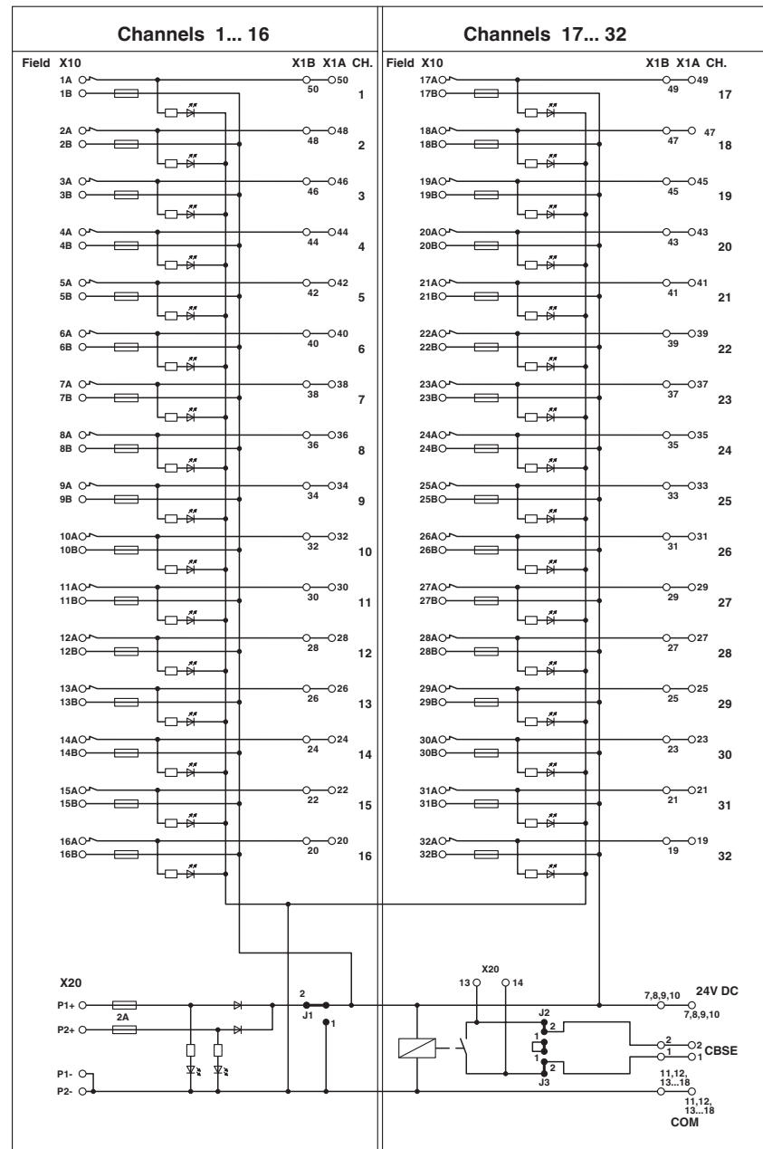
Circuit diagram
