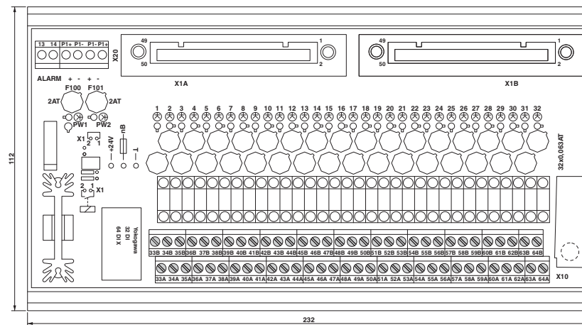
Dimensional drawing
