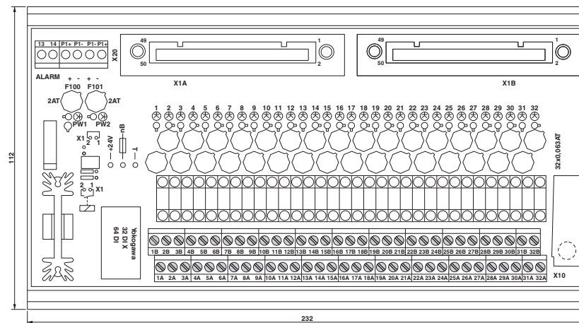
Dimensional drawing
