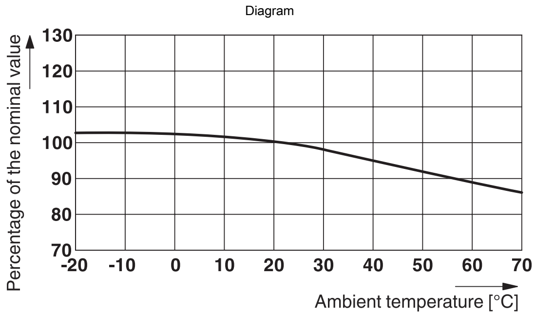
TR5 fuse derating curve
