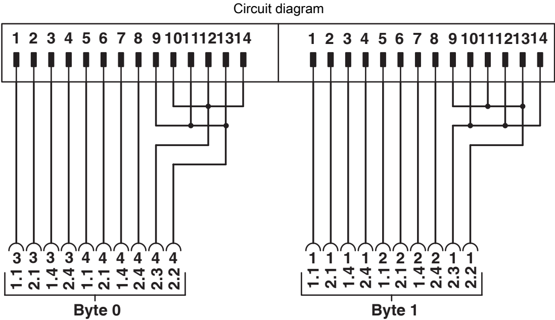
Connection scheme: FLKM 14-PA-INLINE/IN16
