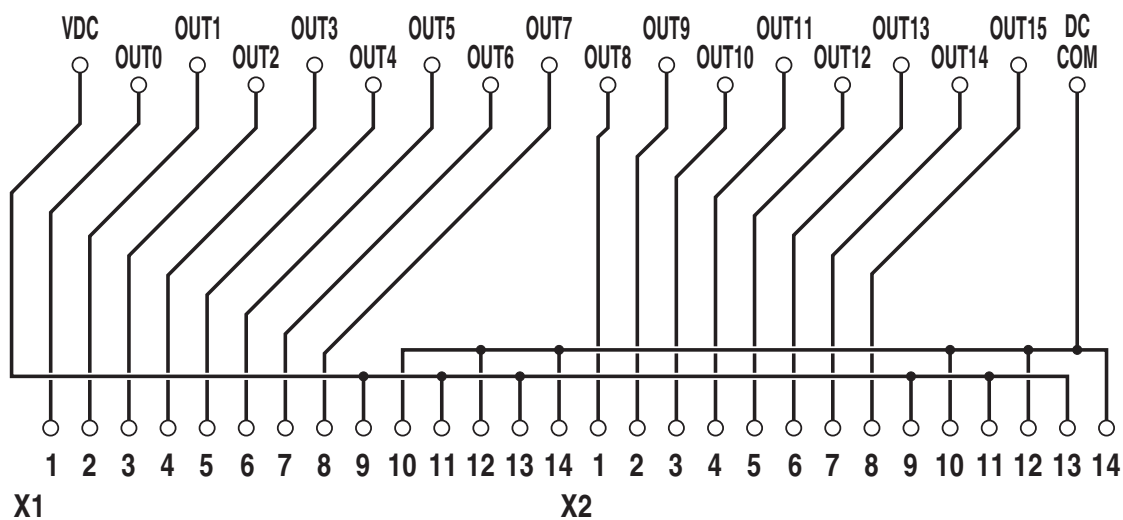
Circuit diagram
