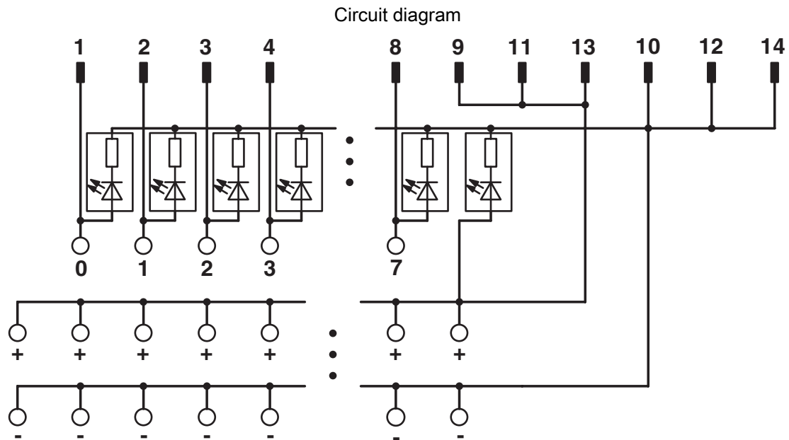
Connection scheme FLKMS 14/8IM/LA/PLC
