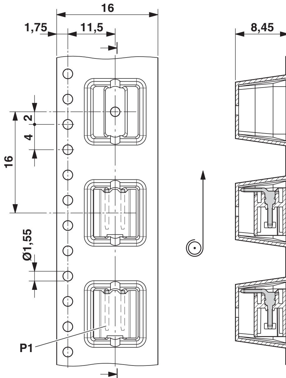
Dimensional drawing
