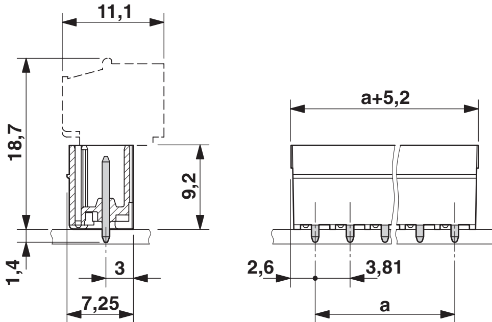
Dimensional drawing
