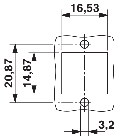
Dimensional drawing
