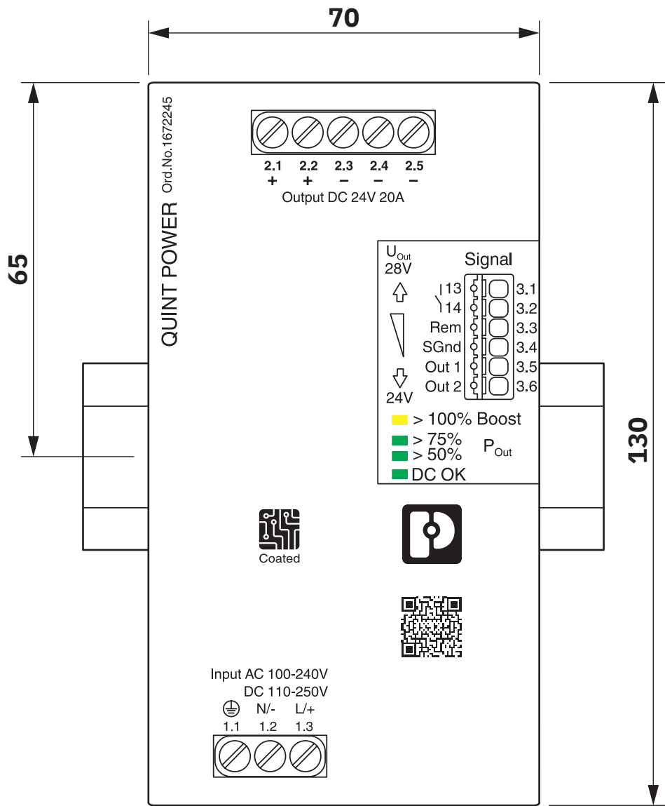
Device dimensions (dimensions in mm)
