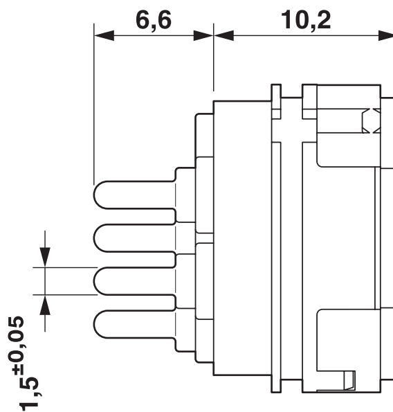
Dimensional drawing
