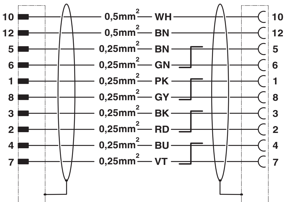
Contact assignment of M23 plugs/sockets
