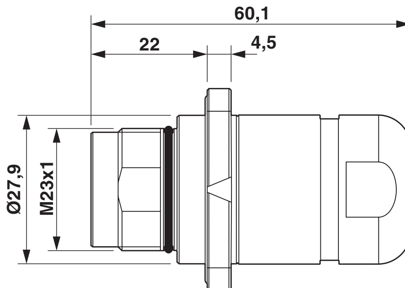
Dimensional drawing
