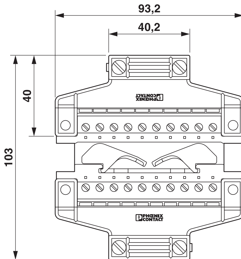
Dimensional drawing
