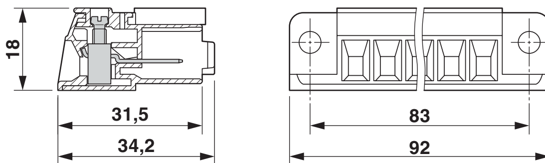
Dimensional drawing
