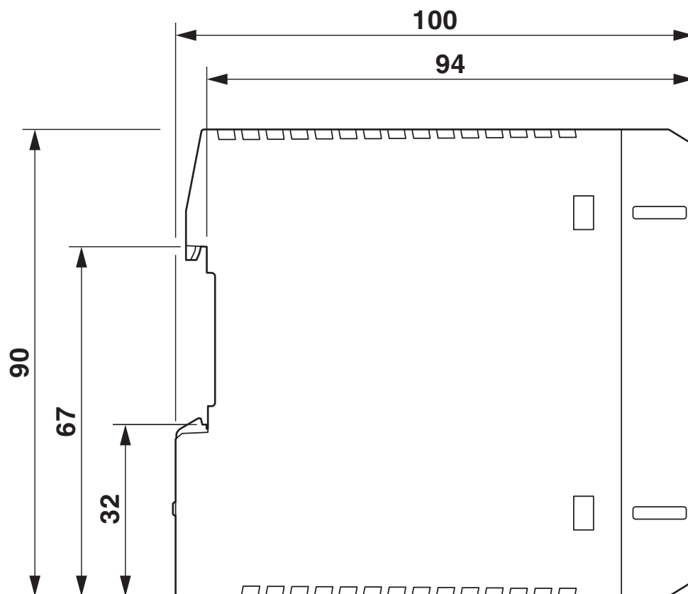
Dimensional drawing
