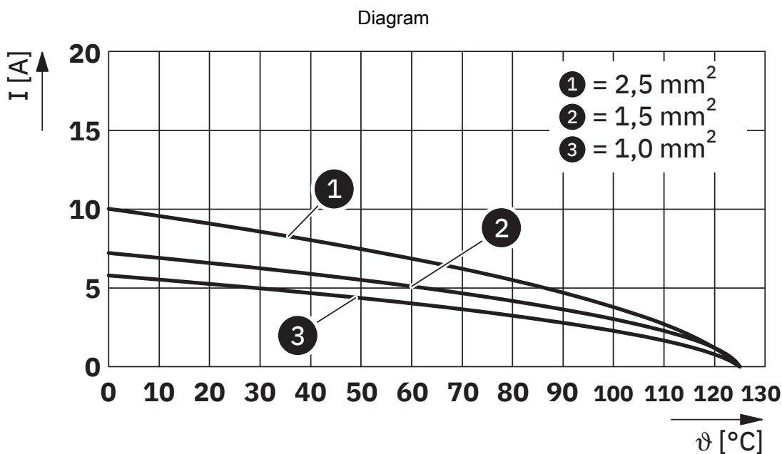
Derating diagram rolled contacts
