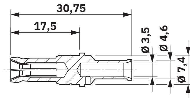
Dimensional drawing
