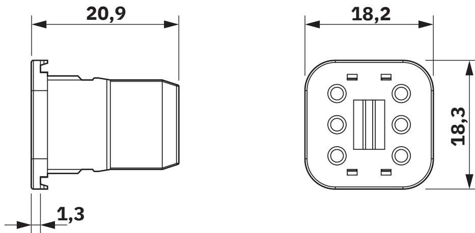
AW6S top view and side view
