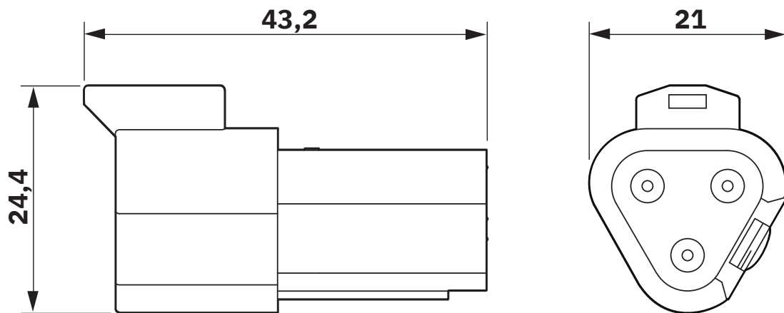
AT04-3P top view and side view
