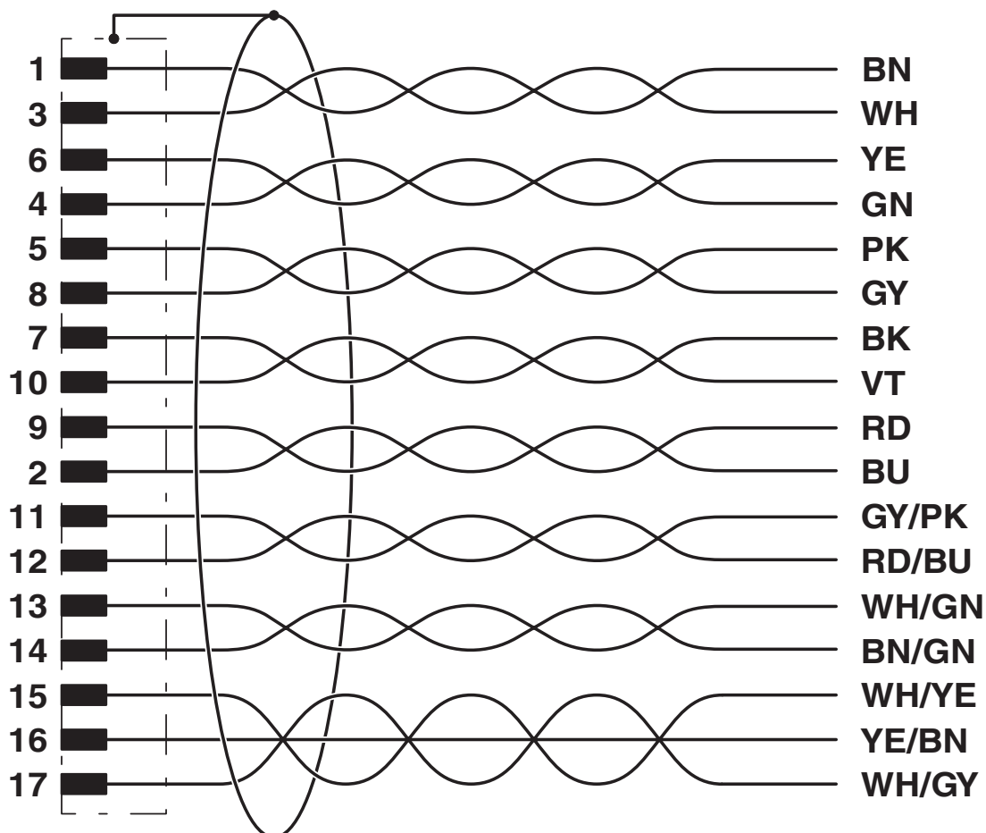
Circuit diagram
