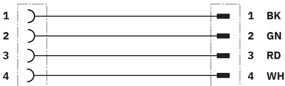
Contact assignment of 1-3/8" plugs/
