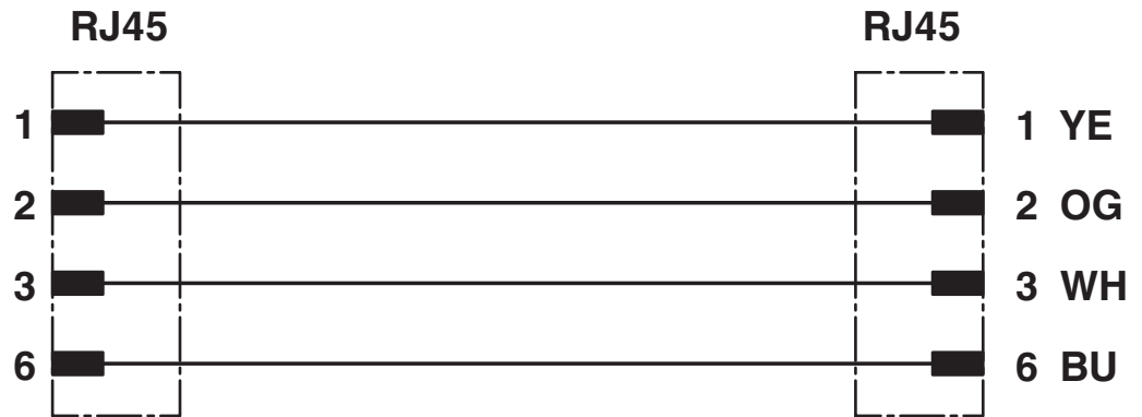
Circuit diagram
