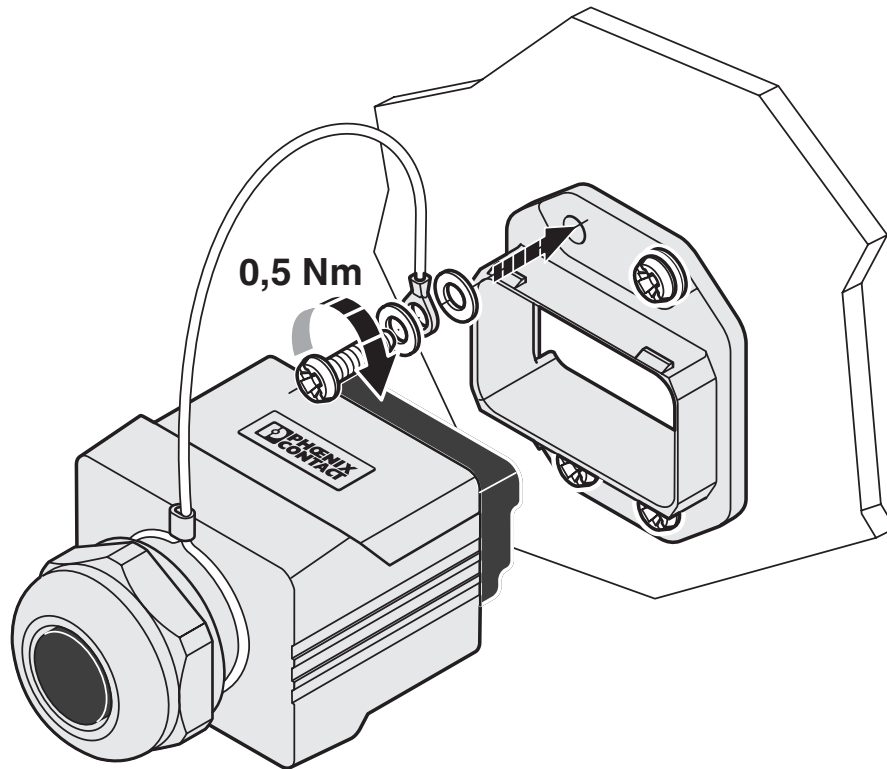
Exploded view
