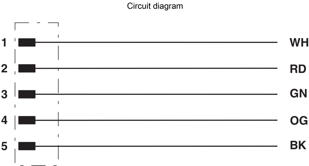
Contact assignment of 7/8" plug
